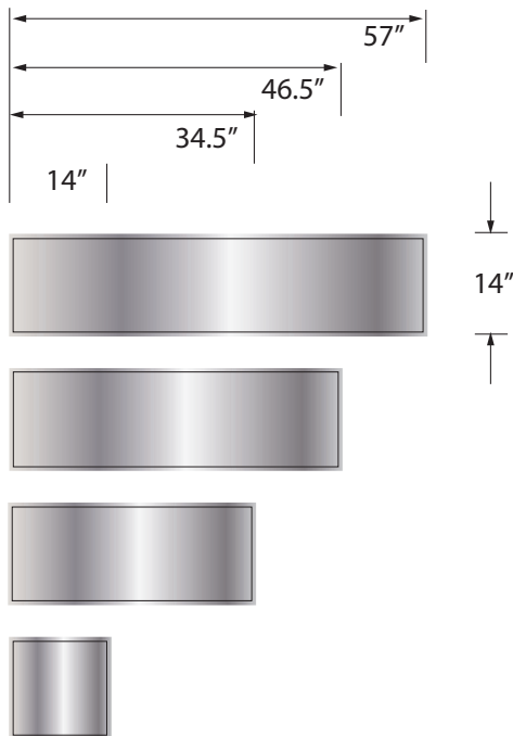
STH / STHL - Horizontal Storage Pods
