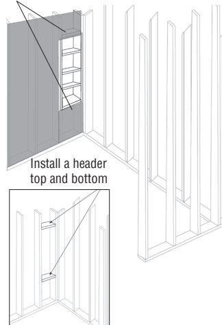
Vertical Storage Box Install a header top and bottom
