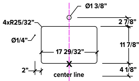
CUTOUT DETAILS
