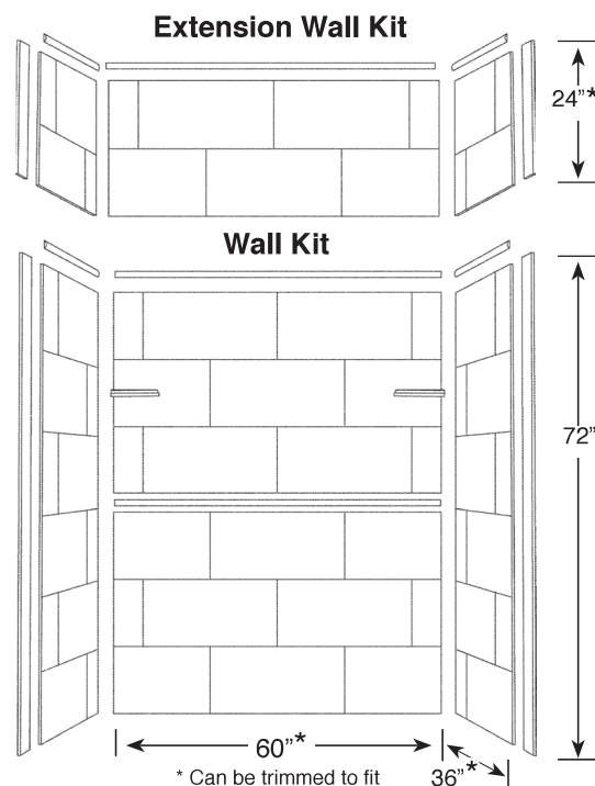
Shown with F6036 Shower Base, X6062 Extension Wall Kit
