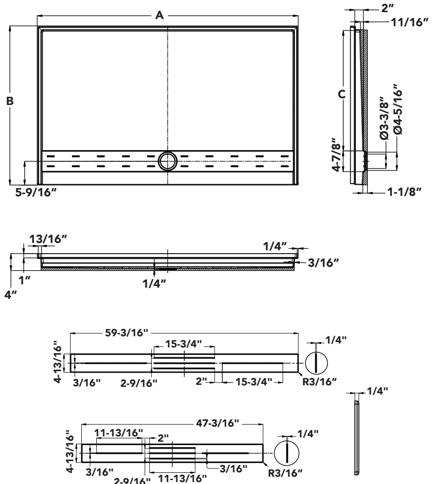
FTD Trench Drain Base
