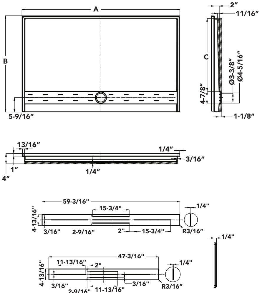
SMFTD Trench Drain Base
