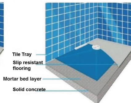
Installation with concrete floors
