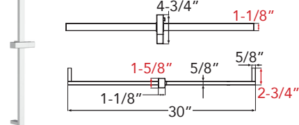
SAMPSON 30" Sliding Bar SMSSSB30-
