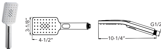
SADIE Three Function Hand Shower SMMHSS3FS-
