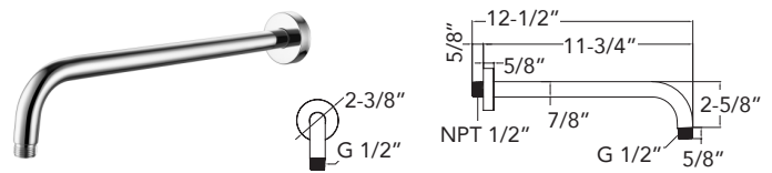
ROWAN 12" Shower Arm SMRSA12-
