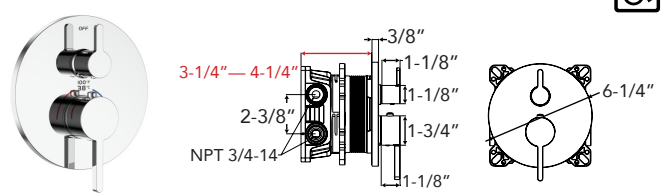
FLOWSTAT Two Function Thermostatic Valve SMVFS2R-
