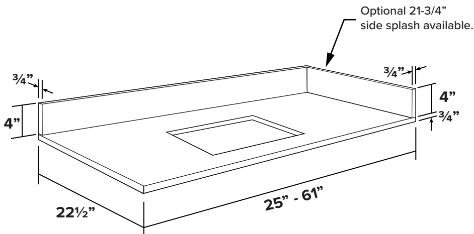
4" Centerset
