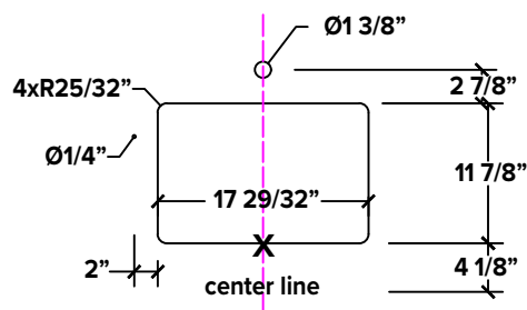
CUTOUT DETAILS
