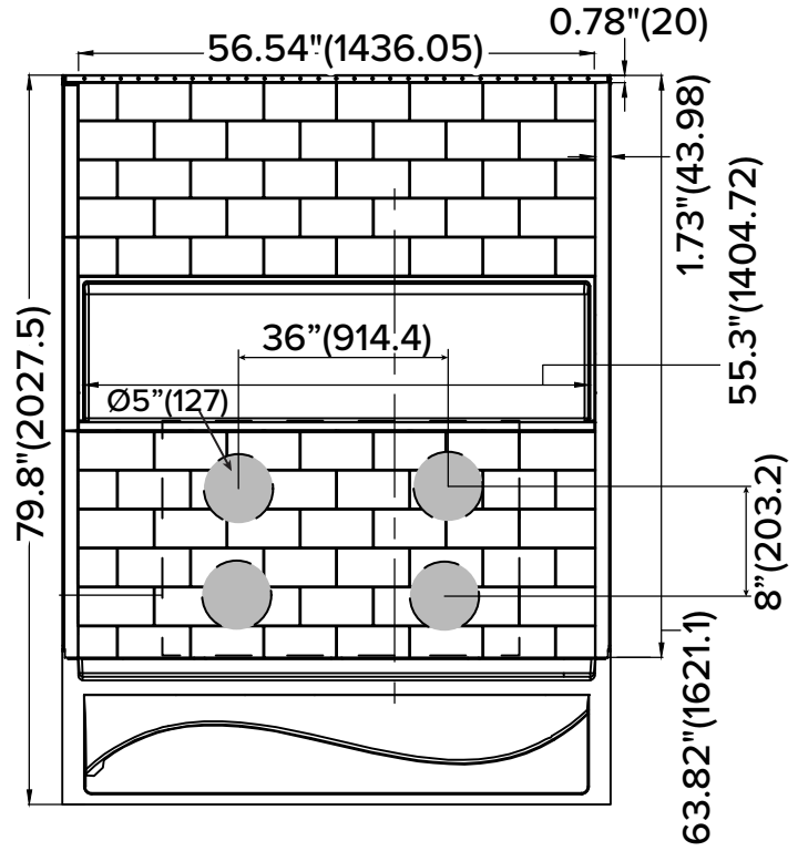
BACKER BOARD LOCATIONS
