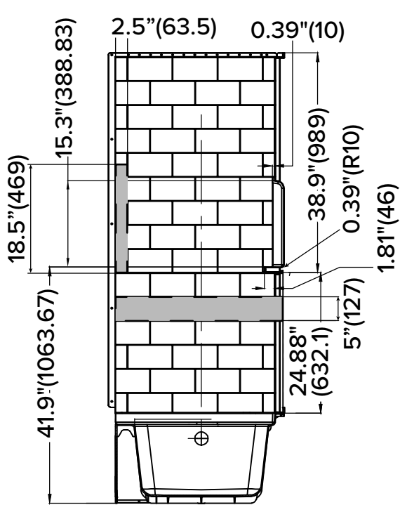
BACKER BOARD LOCATIONS
