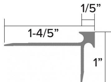
SMTTOCT Outside Corner trim
